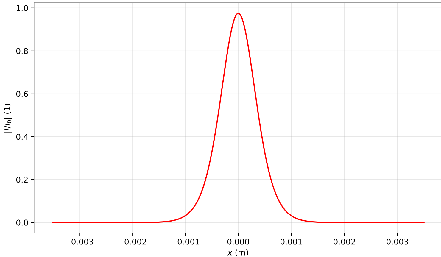
Intensity profile I(x, y = 0, z = 1.433)/I_0 , P_{in}=0.5P_{cr} , artificial time
